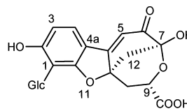
(7S,9S,10aS)-1-β-D-glucosyl-10,10a-dihydro-2,7-dihydroxy-7,10a-methano-6-oxo-9H-8,11-dioxacycloocta[a]indene-9-carboxylic acid
